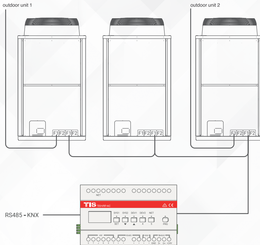
Figure 1: System wiring diagram
